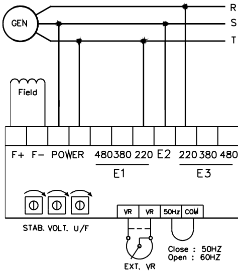
Wiring Diagram Figure 4
