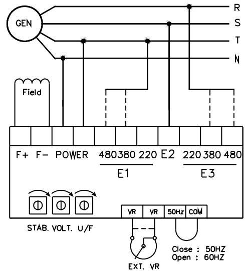
Wiring Diagram Figure 4
